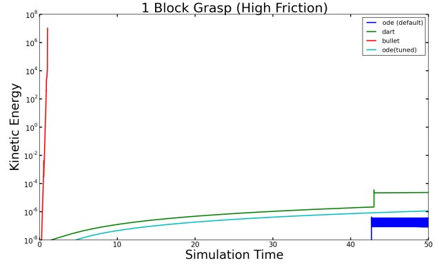
Fig. 3: Metric performance for the multi-block grasping experimental control (using a single block) over three simulators (ODE, BULLET, DART). BULLET becomes unstable immediately. DART (and to a lesser extent, ODE) exhibits a concerning discontinuity in performance, but generally is able to maintain a grasp for the length of the experiment. ODE maintains a stable grasp.
