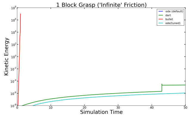
Fig. 5: Metric performance for the multi-block grasping experiment (using a single block) and very high friction value over three simulators (ODE, BULLET, and DART). Performance appears identical to Figure 3.
