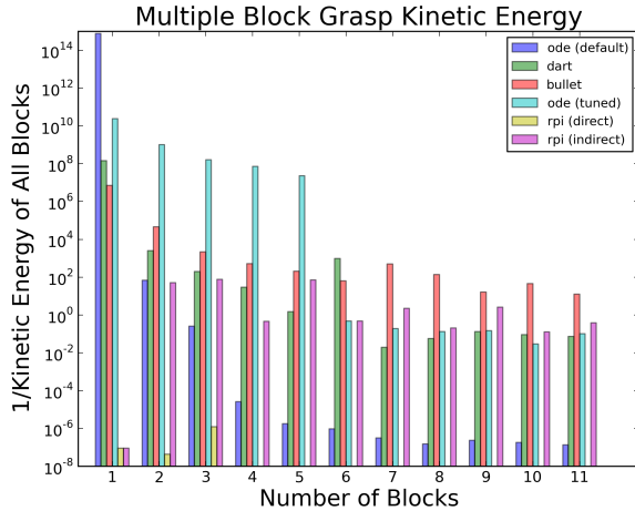
Fig. 6: Logarithmic inverse metric performance for the multi-block grasping experiment, illustrating direct vs. iterative solver performance at the end of 0.3s of virtual time. Taller bars indicate better performance. A missing bar (see, e.g. rpi (direct) for 11 blocks) indicates failure.
